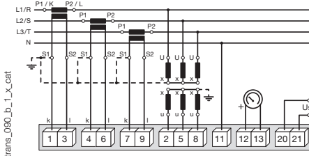
Connections with 3 CT 3 VTs and U_s
