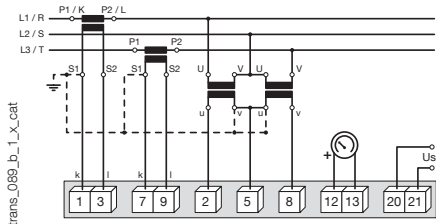
Connections with 2 CT 2 VTs and U_s
