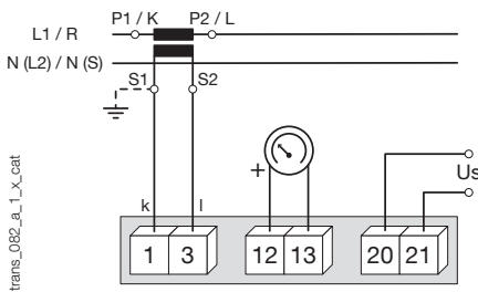
Connections with 1 CT and U_s
