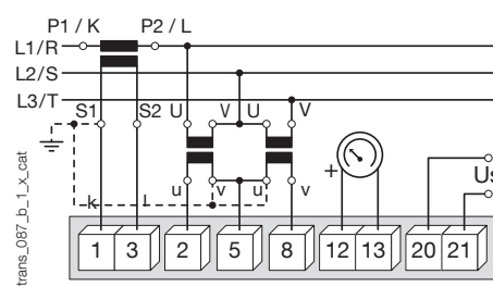
Connections with 1 CT 2 VTs and U_s
