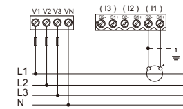
3P4W 1CT Balance load
